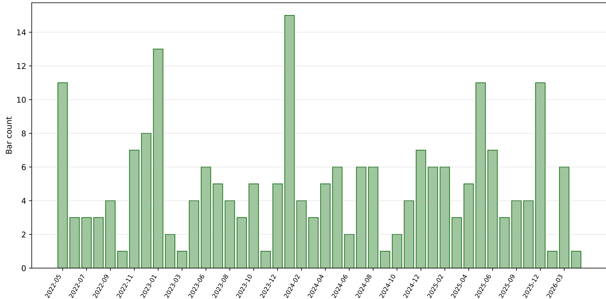
Regime 6 — bar counts by month (UTC, last 44 months) EURUSD · 60-minute bars (H1) · n=25,000 bars
