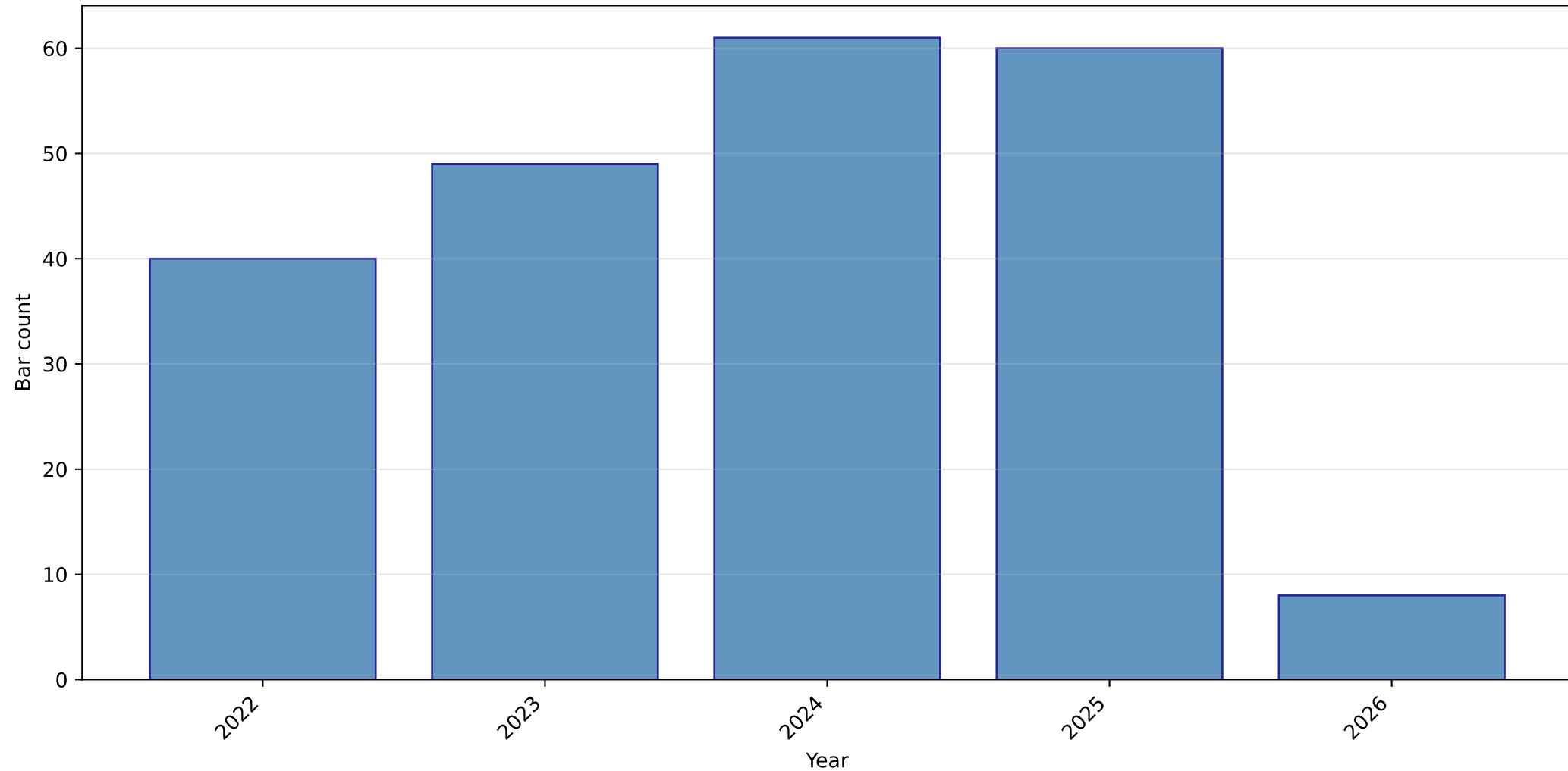
Regime 6 — bar counts by year (UTC) EURUSD · 60-minute bars (H1) · n=25,000 bars
