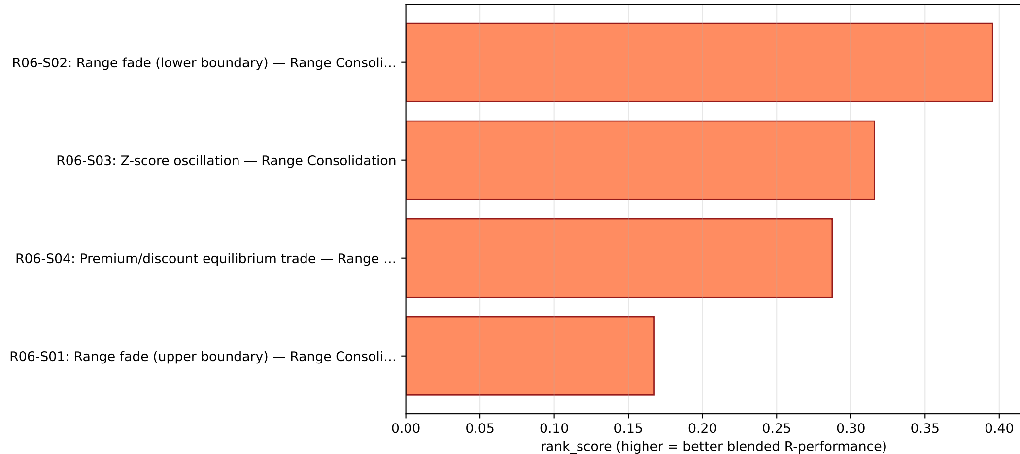
Top strategies by rank_score — regime 6 EURUSD · 60-minute bars (H1) · n=25,000 bars
